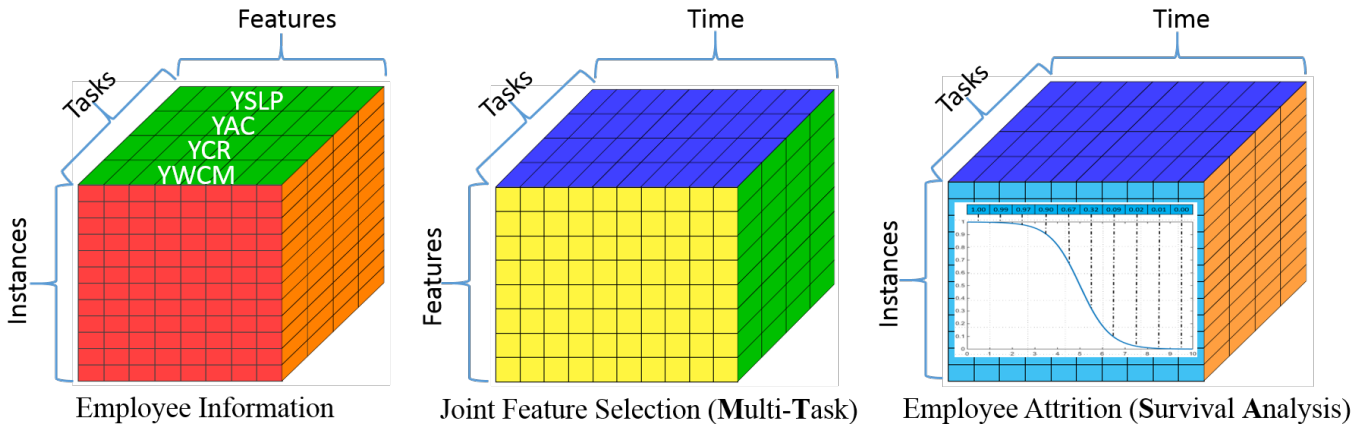
Fig. 1: An illustration of various components in the proposed MTMT framework using Employee Attrition dataset.
