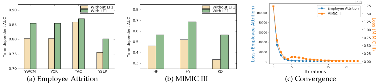
Fig. 3: Effect of \ell_{F,1} norm on feature selection for both (a) employee attrition and (b) MIMIC III. (c) Convergence of MTMT model on both datasets.
