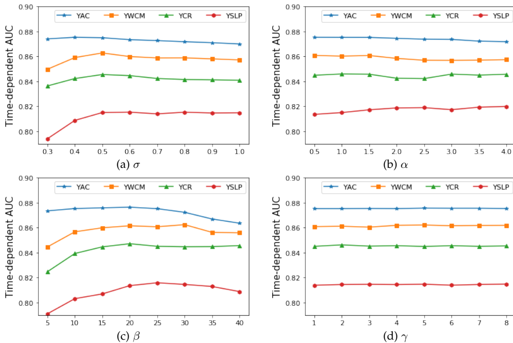
Fig. 4: Parameter sensitivity of the four parameters used in the proposed method on Employee Attrition dataset.
