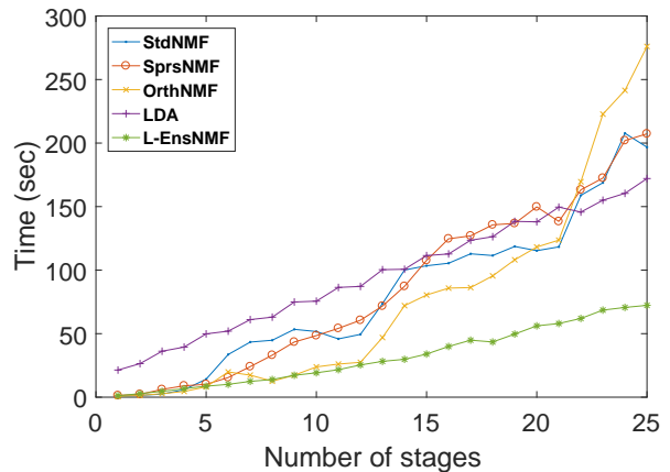
Figure 4: Comparison of computing times for VisPub dataset. The results were obtained from the average values over 50 runs.
