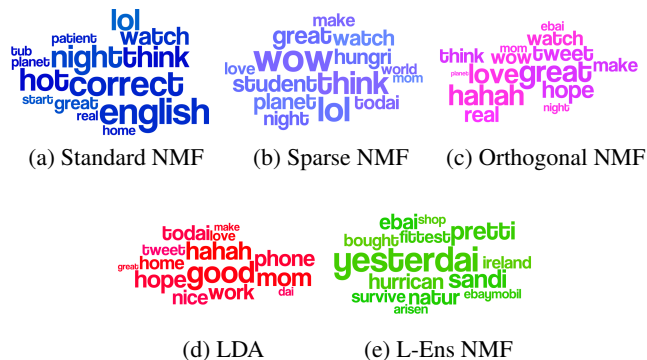
Figure 1: Topics computed from Twitter dataset
