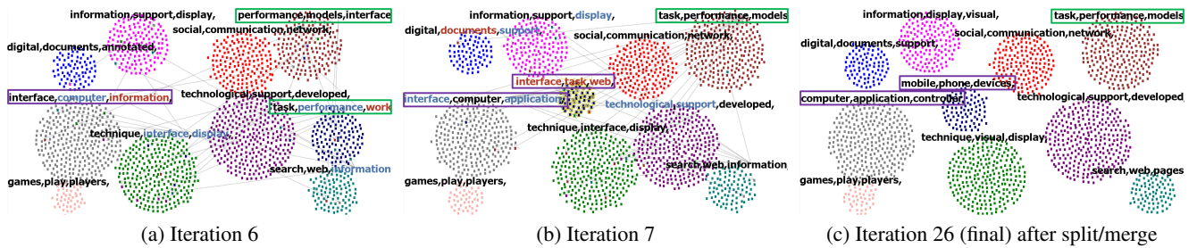
Figure 8: Split and merging interactions with k -means. From (a) to (b), the green clusters are merged and the purple cluster is split at the sixth iteration. The final result is in (c). The CHI papers published from 1999-2010 were used.
