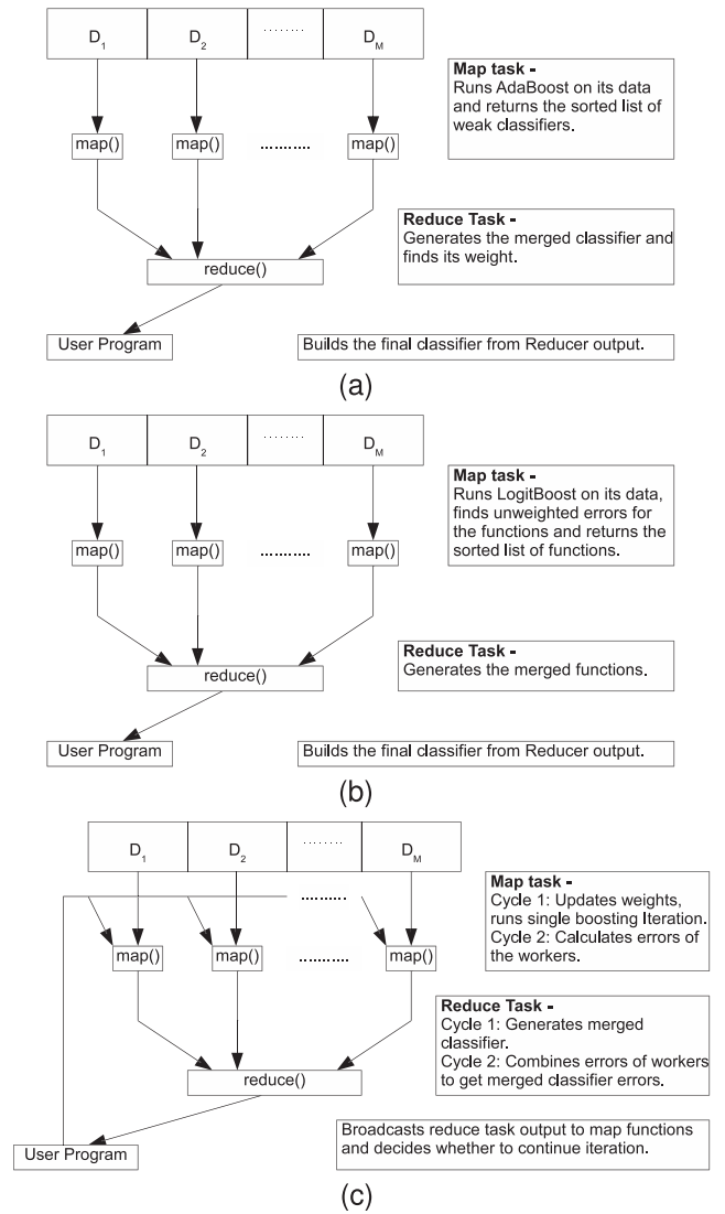
Fig. 1. MapReduce work flow for: (a) ADABOOST.PL, (b) LOGITBOOST.PL, and (c) MULTBOOST.
